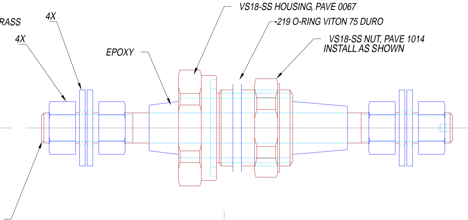
1/2 FLAT WASHER, BRASS
