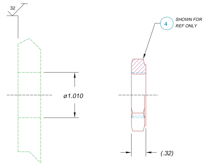
LEAK TEST PORT OR INSTALLATION
