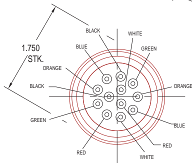
APPROXIMATE WIRE LOCATIONS
