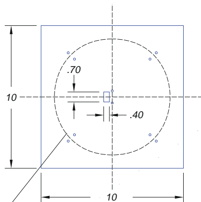
CARDBOARD SHIPPING VEHICLE SCALE 1 = 5
