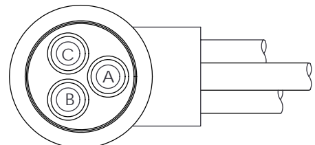
MATING FACE VIEW
