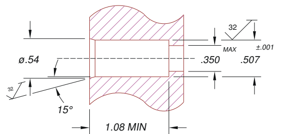
LEAK TEST PORT REFERENCE ONLY
