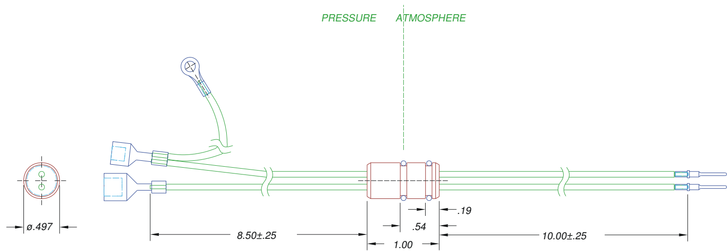
LEAK TEST PORT REFERENCE ONLY
