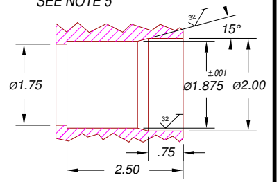
LEAK TEST PORT DIMS SCALE 1=2 SEE NOTE 5
