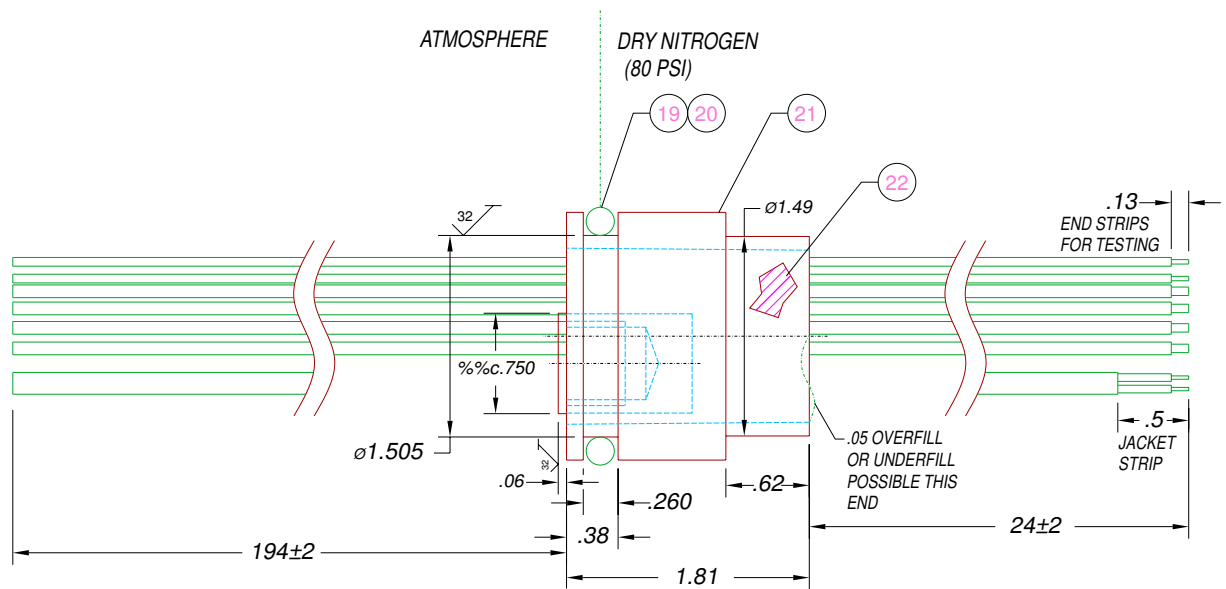
LEAK TEST PORT DIMS SCALE 1=2 SEE NOTE 5
