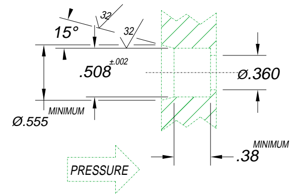
LEAK TEST PORT
