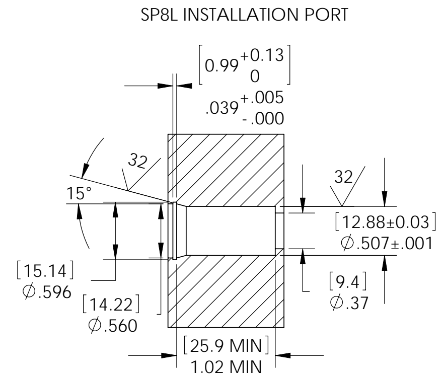
RECOMMENDED RETAINING RING TRUARC #5000-56 OR EQUAL
