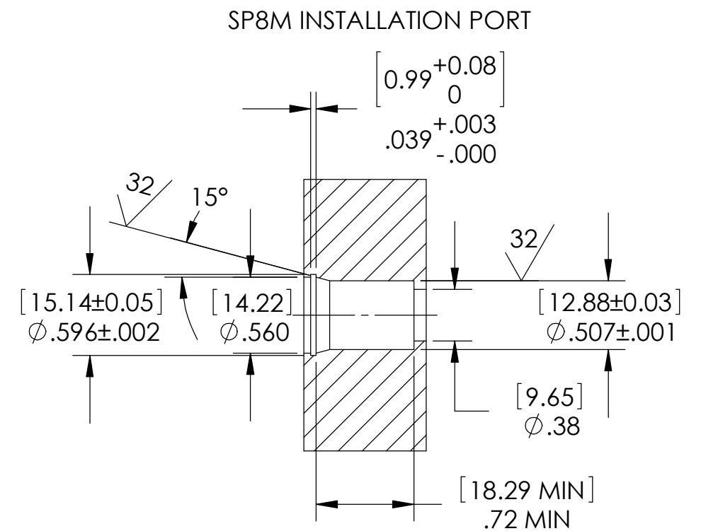
RECOMMENDED RETAINING RING TRUARC N5000-56 OR EQUAL
