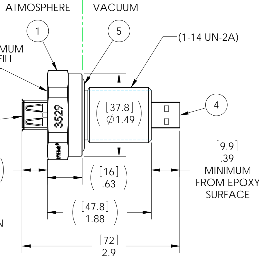
VACUUM / MALE PIN LOCATION SCALE: 3:1
