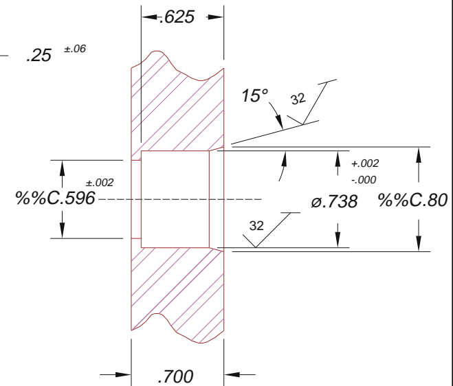
LEAK TEST PORT SHOW FOR REFERENCE ONLY
